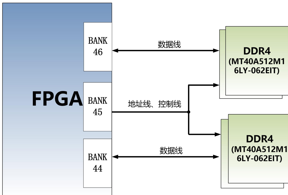
Figure 3-1 DDR4 DRAM
