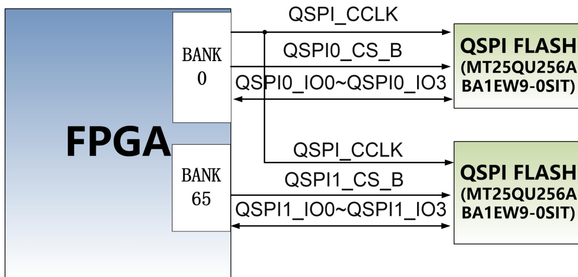
Figure 4-2 QSPI Flash
