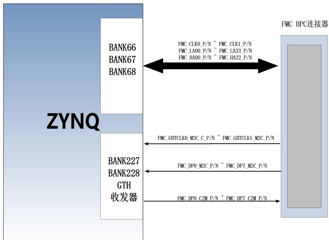
Figure 10-3 HPC FMC3
