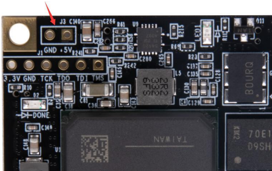
Figure 2-9-2: J3 interface on the Core Board
