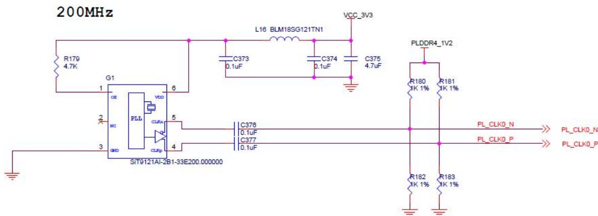
Figure 2-6-4: PL system clock source
